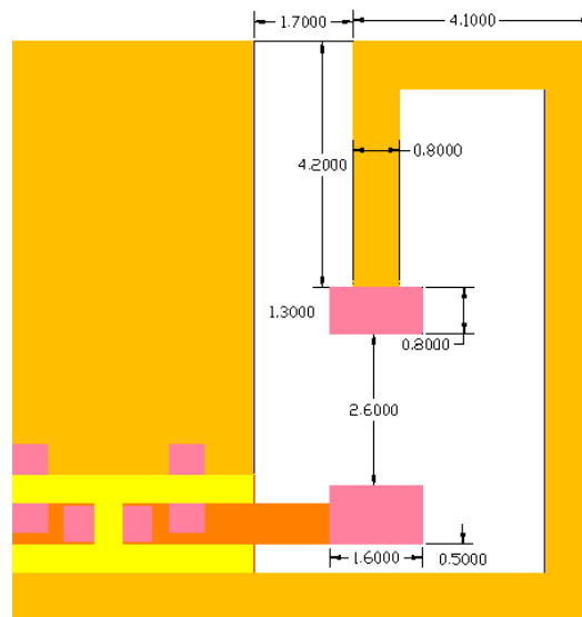
Layout Dimensions in Clearance area( Size=5.8*9.9mm)
